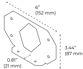
Data hub stack mount
