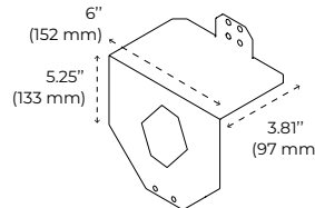
Power Supply Upper
